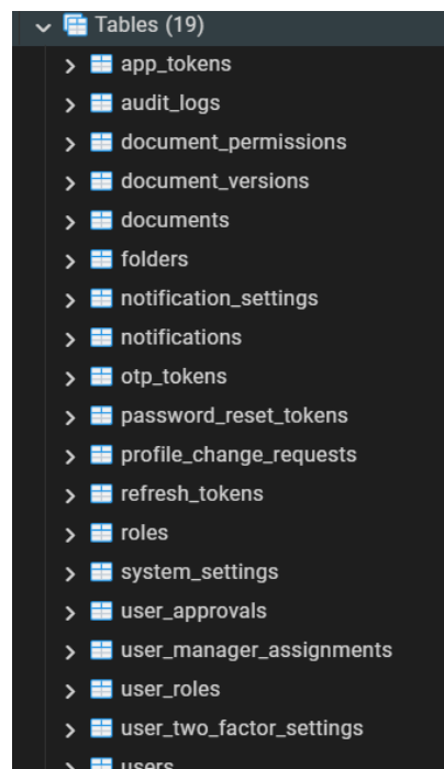
Figure 13: Database Schemas
