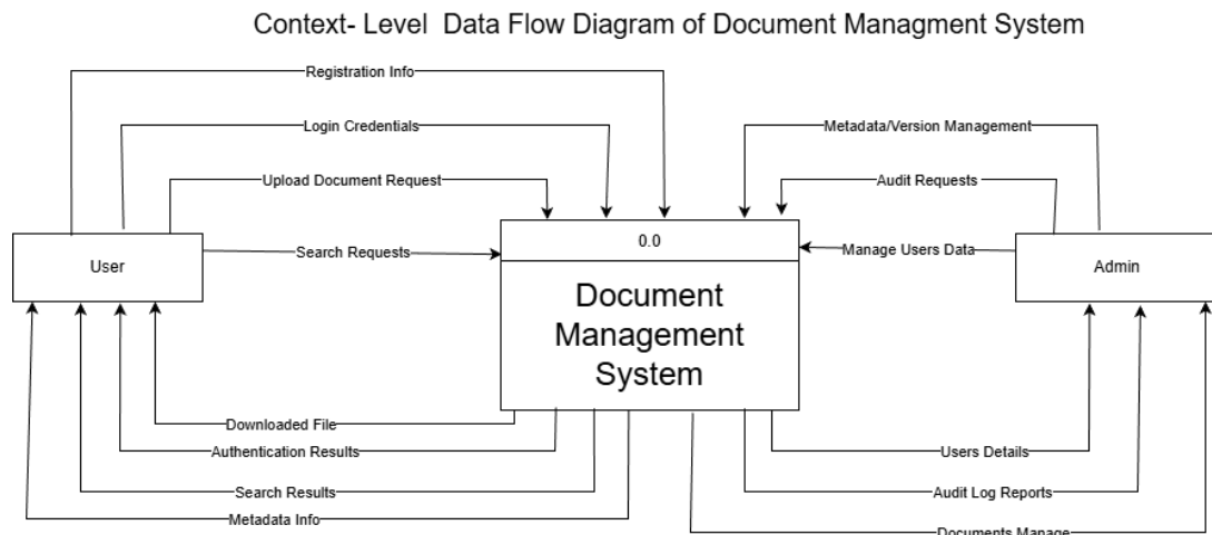
Fig. 2: Context Diagram
