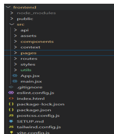
Figure 11: Frontend structure
