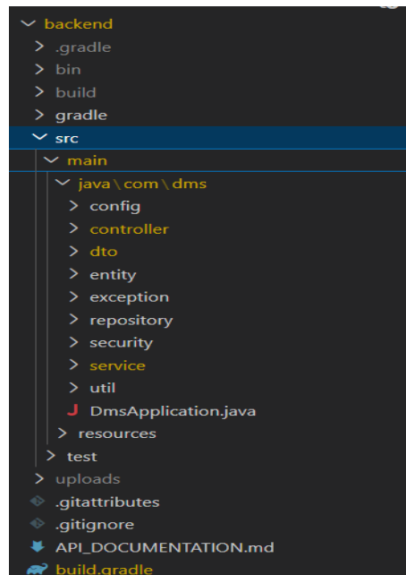
Figure 12: Backend structure
