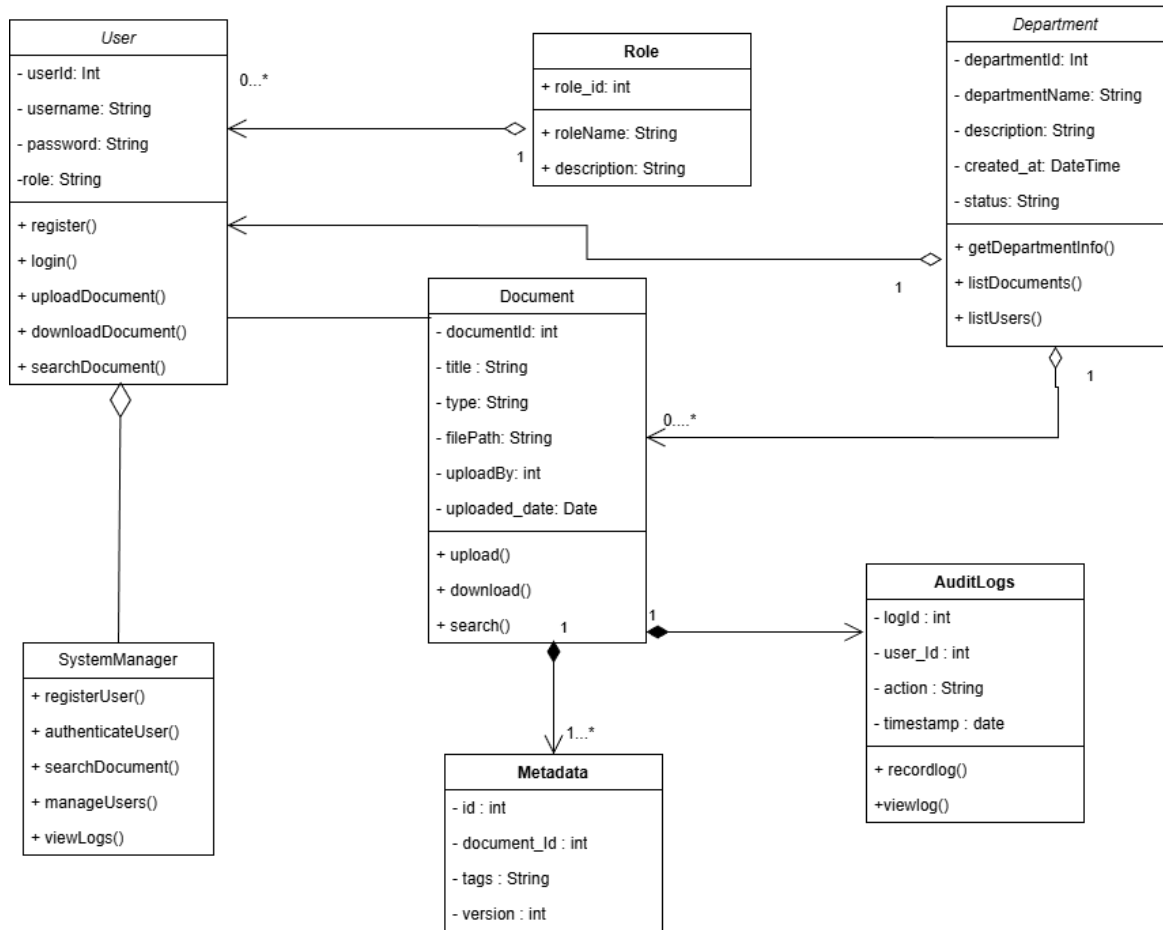
Fig. 6: Class Diagram
